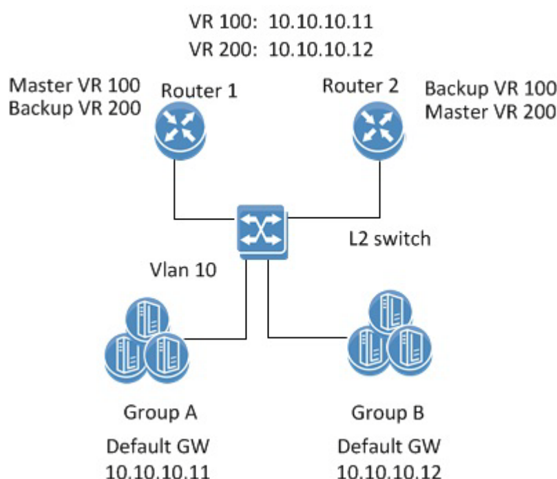
Figure 31: Common VRRP Configuration with Load Balancing
