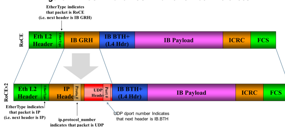
Figure 24: RoCEv2 and RoCE Frame Format Differences
