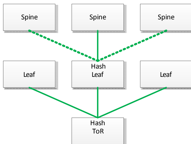
Figure 27: Multiple Hash Functions
