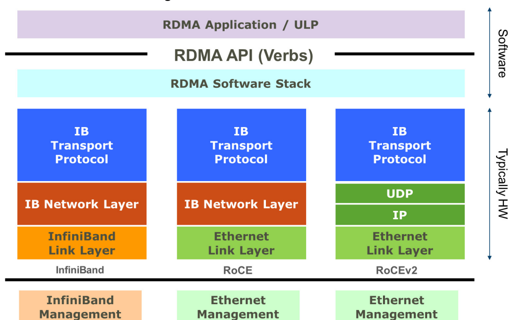
Figure 25: RoCEv2 Protocol Stack
