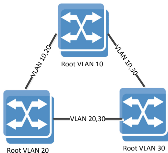
Figure 17: RPVST Network Config
