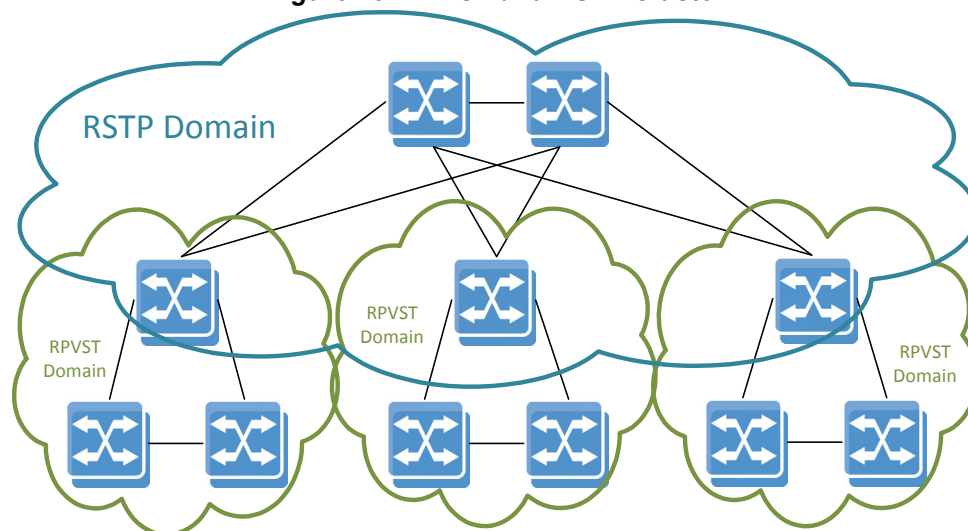
Figure 18: RPVST and RSTP Cluster
