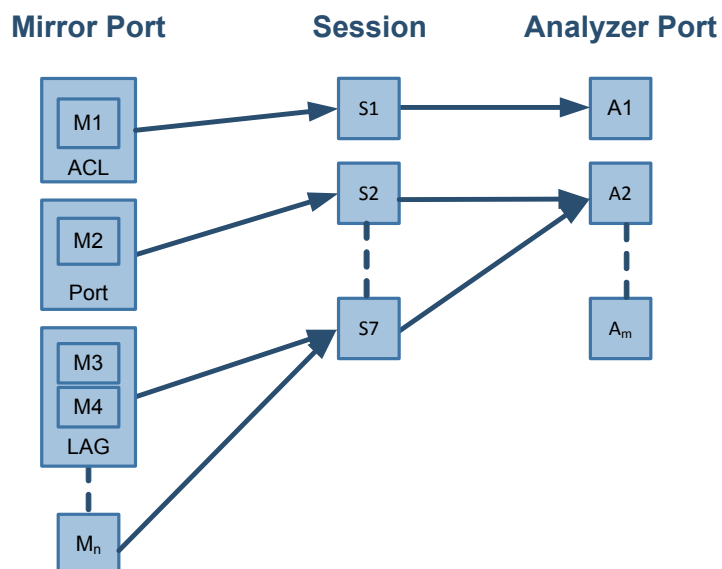
Figure 20: Mirror to Analyzer Mapping
