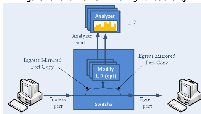
Figure 19: Overview of Mirroring Functionality
