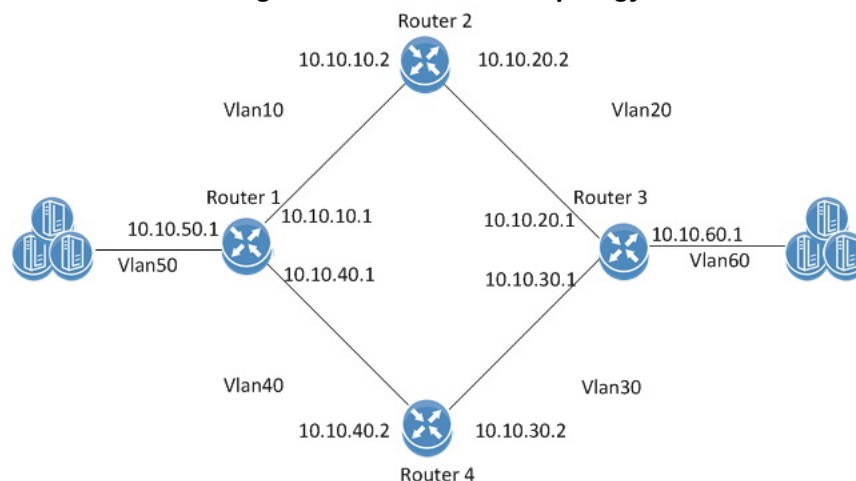
Figure 29: OSPF Basic Topology
