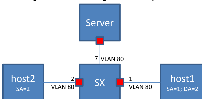
Figure 16: MAC Learning Disable Example Case
