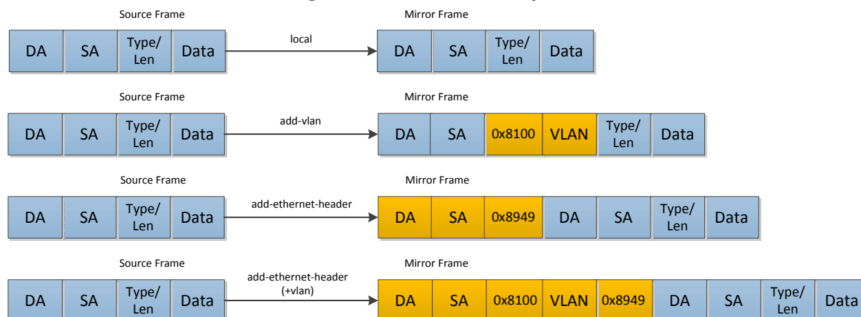
Figure 21: Header Format Options
